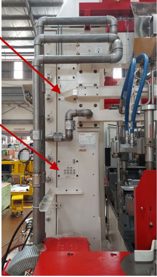
MCU connections to overhead functions
